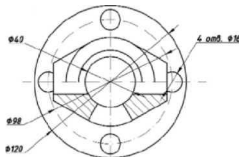
Figure 4. Finished drawing of a part of the "Housing" type.
