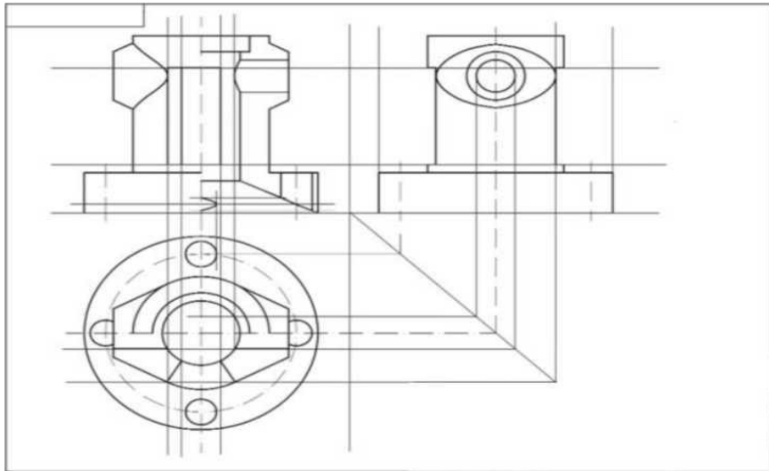
Figure 3. Construction of intersection lines.
